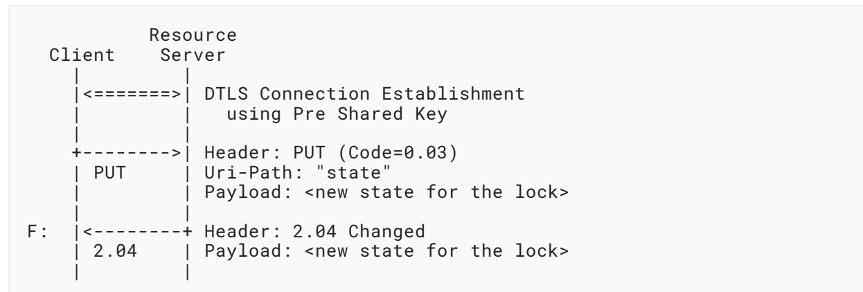
Figure 20: Resource Request and Response Protected by OSCORE
