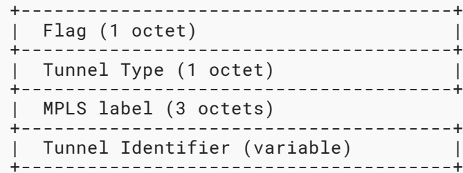
Figure 9: PMSI Tunnel Attribute
