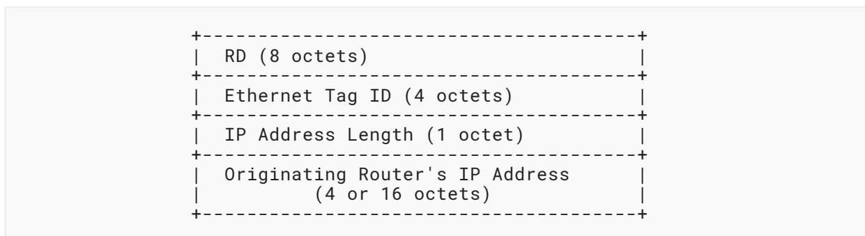
Figure 8: EVPN Route Type 3
