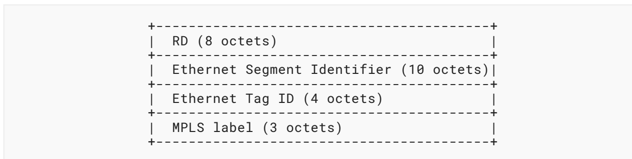
Figure 6: EVPN Route Type 1
